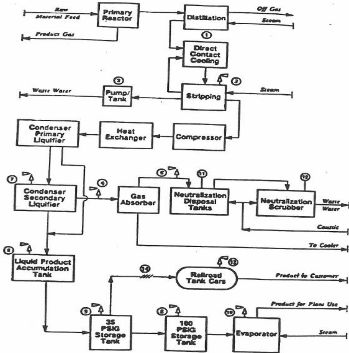
EXAMPLE OF A BLOCK FLOW DIAGRAM
