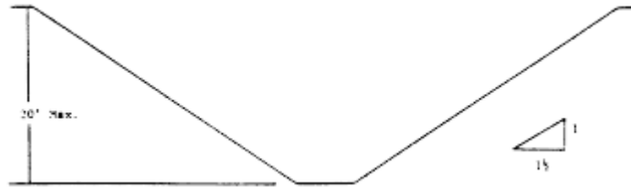
Simple Slope
