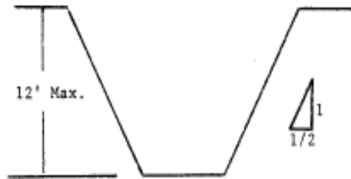
Simple Slope—Short Term
