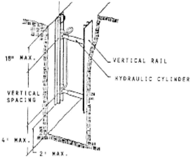
Figure 1. Aluminum Hydraulic Shoring
