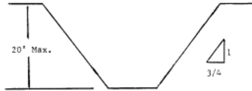
Simple Slope—General
