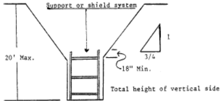
Supported or Shielded Vertically Sided Lower Portion
