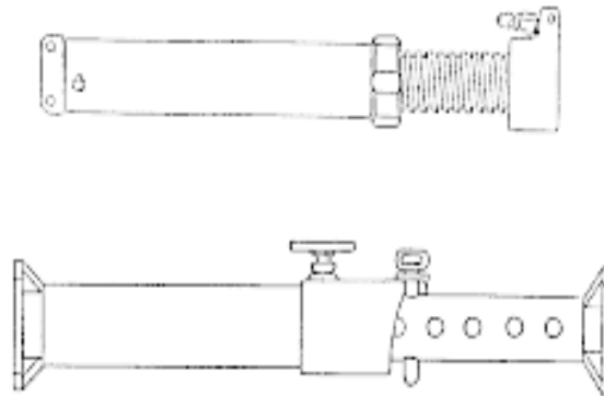
Figure 2. Pneumatic/hydraulic Shoring
