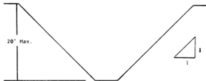
SIMPLE SLOPE
