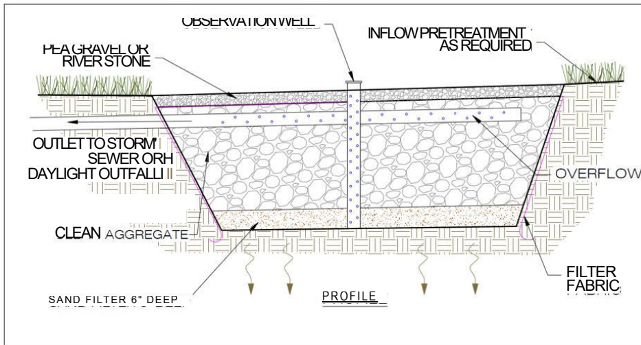
Figure P-FIL-04-6 Typical Infiltration Trench
