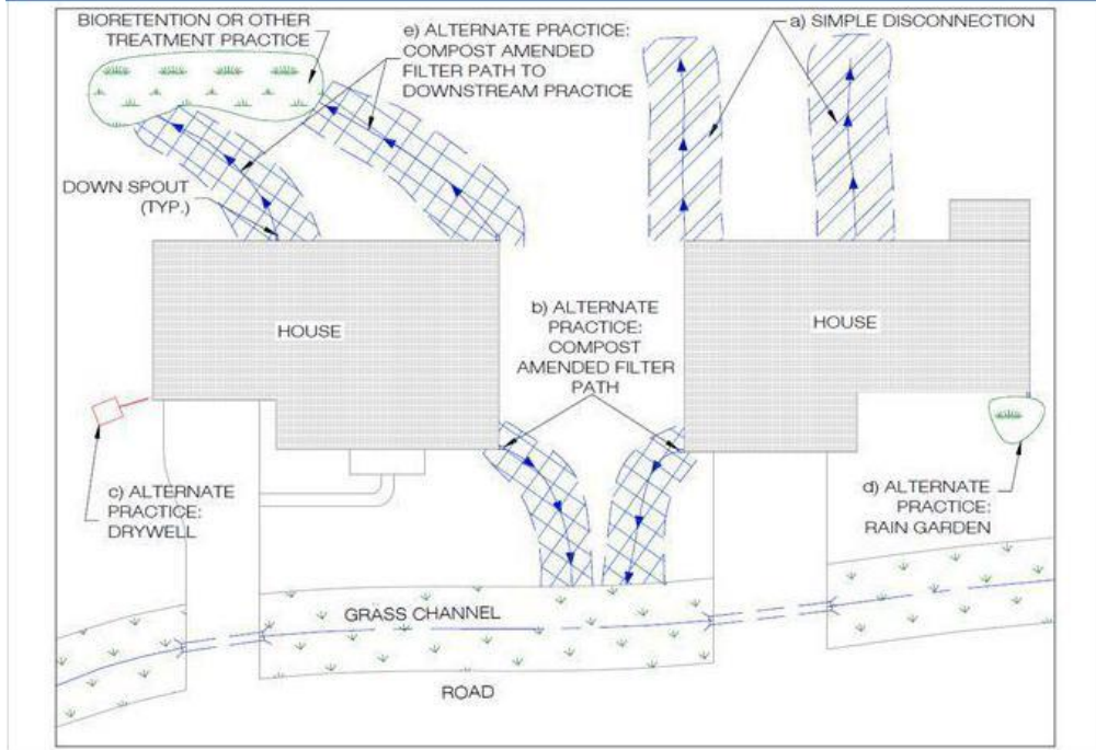
Figure P-FIL-01-1 Roof Disconnection with Alternate Runoff Reduction Practices – Plan View
