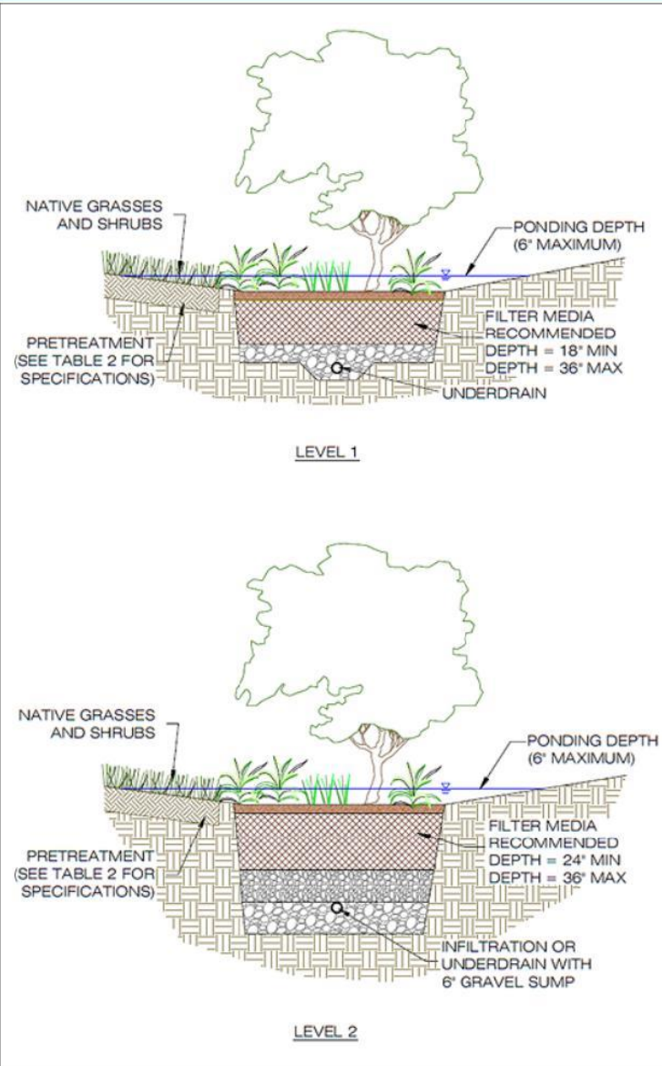
Figure P-FIL-01-7.6 Disconnection: Alternate Practice Rain Garden (Micro Bioretention)
