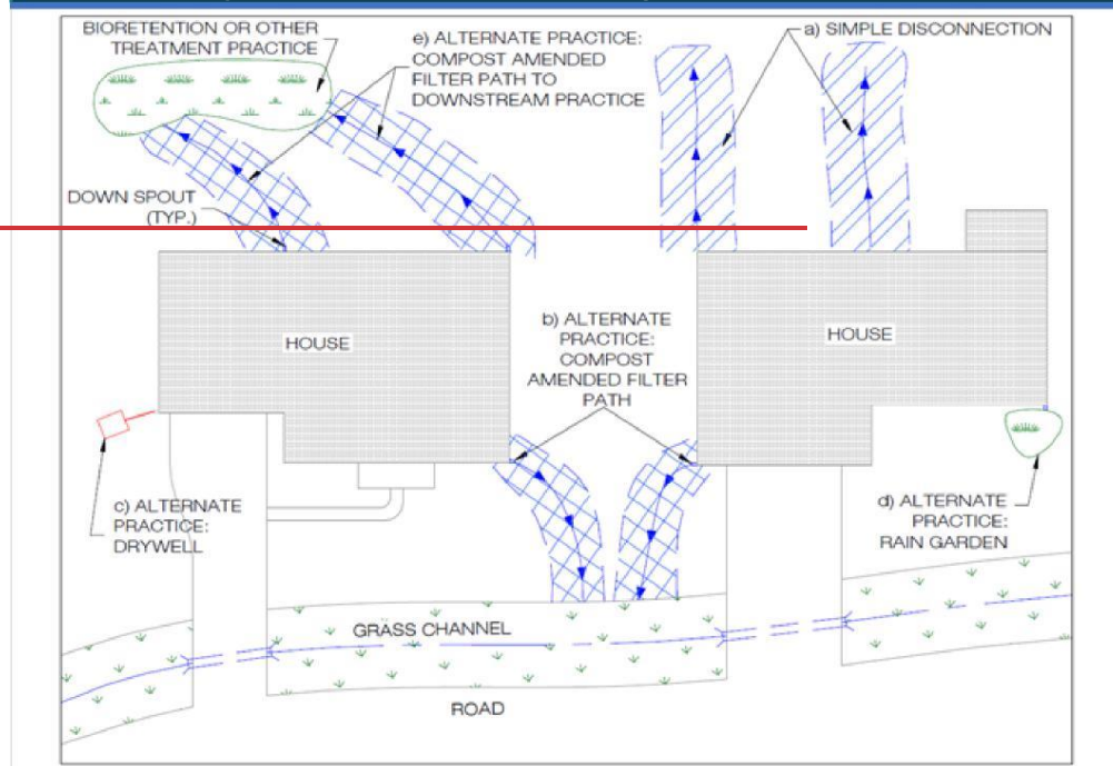
Figure P-FIL-01-2 Residential Rooftop Treatment – Plan View
