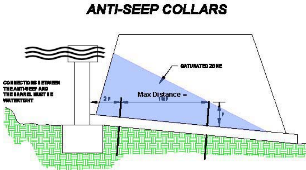
Figure 7-16: Anti-Seep Collars
