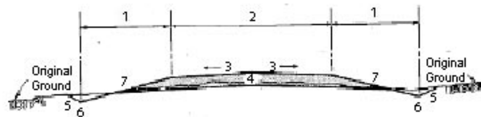
TYPICAL FILL SECTION
