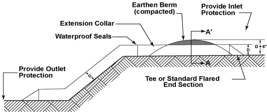
SECTION VIEW
