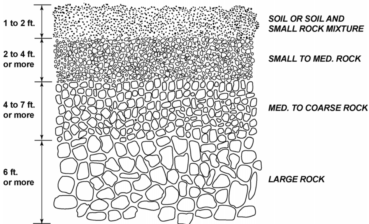
Suggested layering of different size spoil material for revegetation of surface mine spoils.
