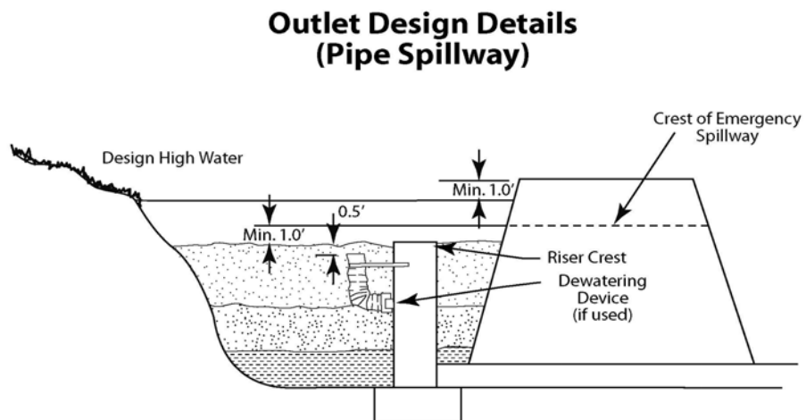
Design Elevations with Emergency Spillway
