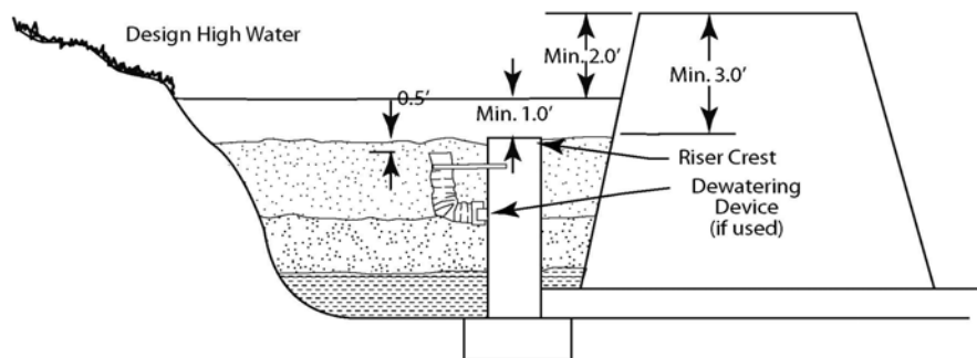
Design Elevations without Emergency Spillway
