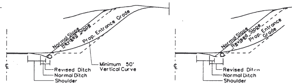
ALTERNATE METHODS FOR PLACING PIPES UNDER ENTRANCES
